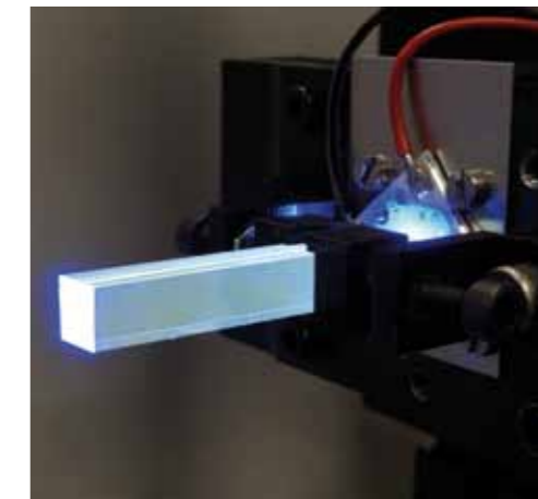
Dy 3+ -doped light rod which conducts the light generated under blue excitation.
